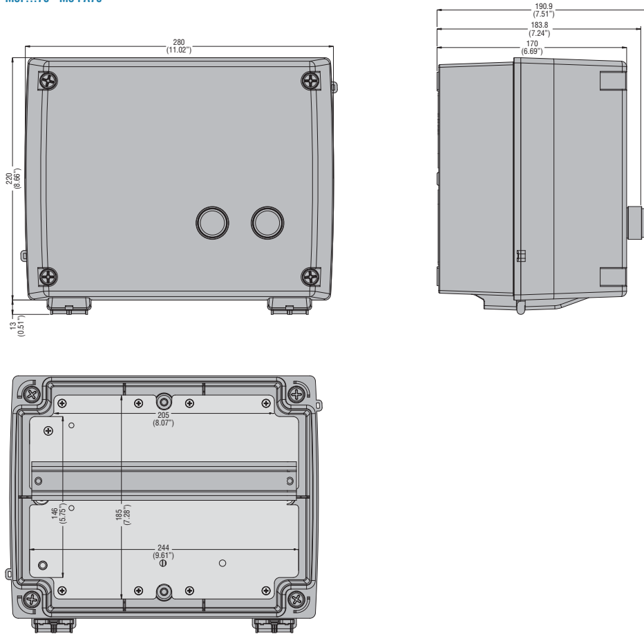
STAR-DELTA STARTERS IN ENCLOSURE - EMPTY ENCLOSURE FOR STAR-DELTA STARTERS M3P...70 - M3 PA70
