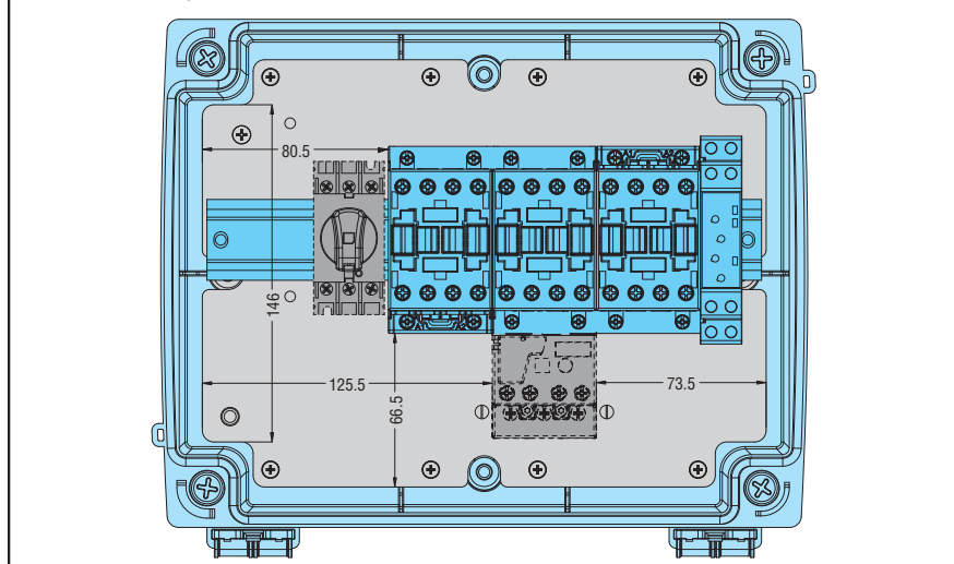
Maximum available space inside M3P... star-delta starters and M3 PA70 enclosure
