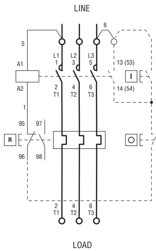
Diagram 2 - External button control
