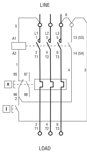
Diagram 1 - Incorporated button control
