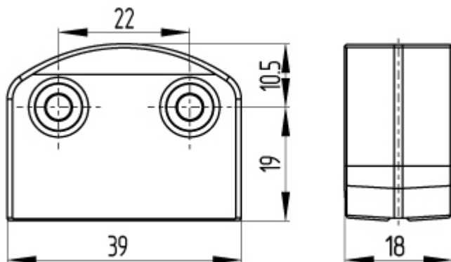
Dimensional drawing (actuator)
