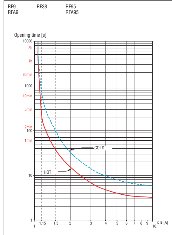
Two-phase operation (phase failure/single phase)
