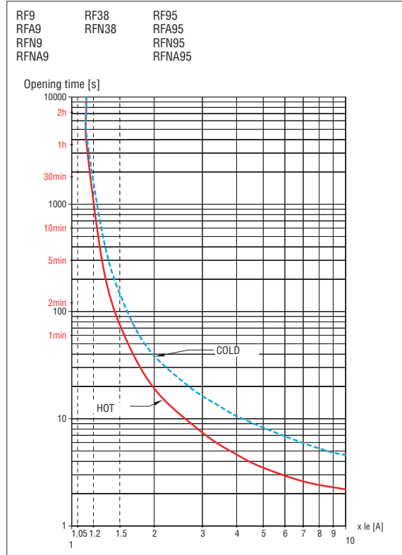
TRIP CHARACTERISTIC FOR RF THERMAL OVERLOAD RELAYS (AVERAGE TIME) Three-phase balanced operation
