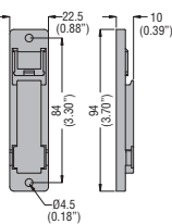
CE106 adapter
