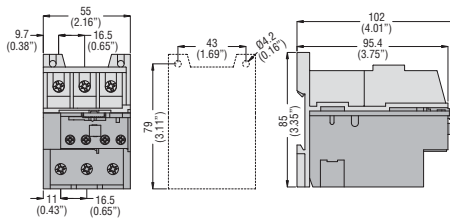
G270 base c/w RF...95 thermal relay
