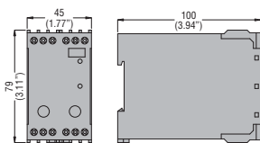
DRPT relay
